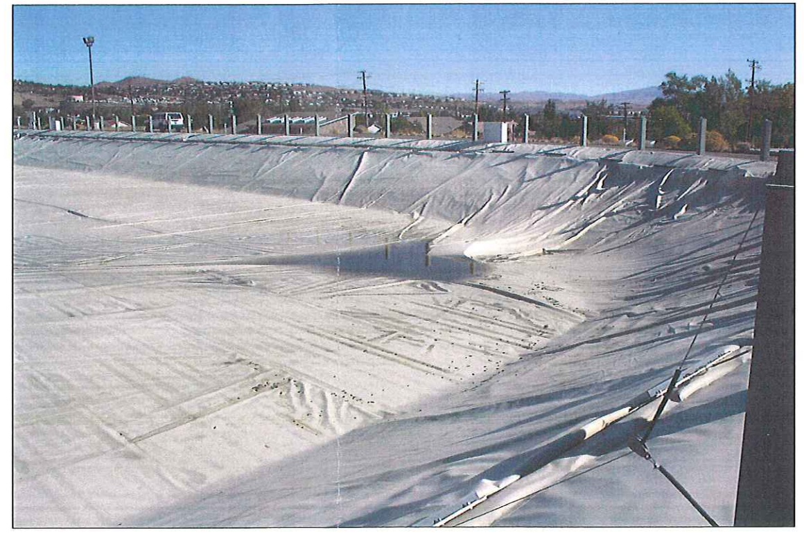
NORTH EAST COVER CORNER -- NO SCALE
